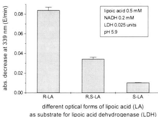
Fig. 1. Oxidation of NADH by lipoic dehydrogenase with different optical forms of lipoic acid as substrate. The measured activity of LDH (based on the molar extinction coefficient \epsilon = 6200 for NADH) was for R -LA as substrate 0.0135 \pm 0.0005 units, for the racemate R,S -LA 0.0055 \pm 0.0003 units and for S -LA as substrate 0.0016 \pm 0.0002 units.
